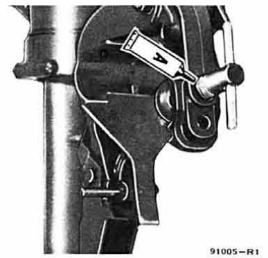
Figure 2-5. Clamp Screw Lubrication
