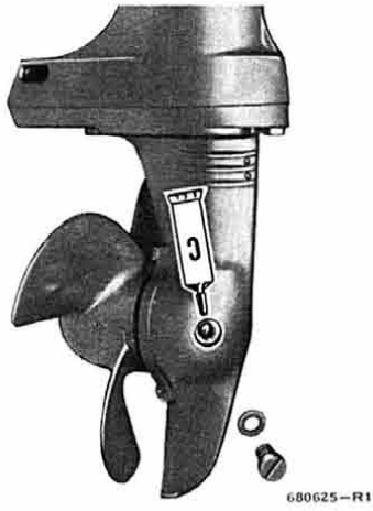
Figure 2-2. Gearcase Lubrication
