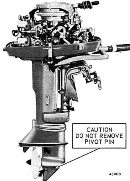
Figure 2-1. Starboard Side
