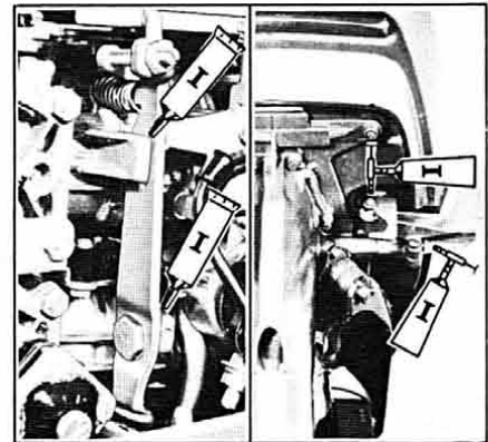
Figure 2-9. Gear Shift Lever Shaft & Lockout
