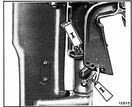
Figure 2-7. Swivel Bracket Fittings & Reverse Lock
