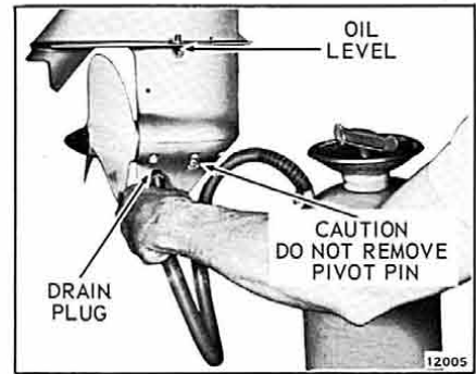
Figure 2-8. Gearcase
