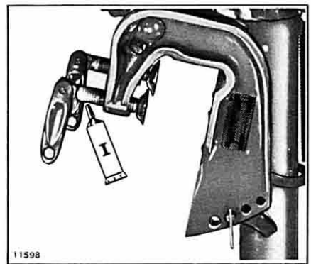
Figure 2-10. Clamp Screws
